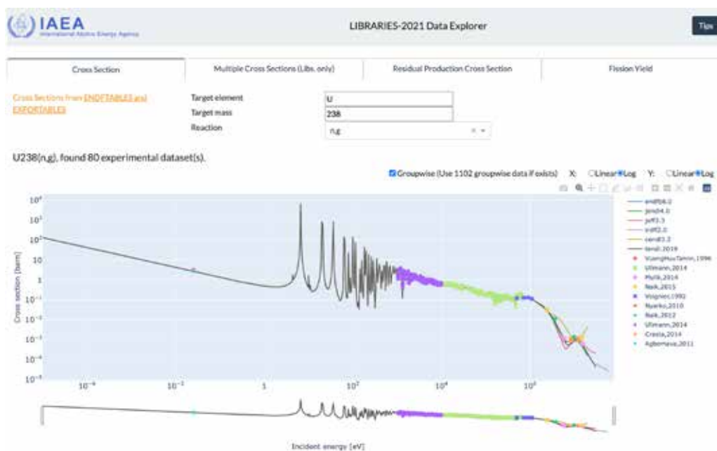
FIG. 1. The Libraries-2021 Data Explorer for retrieval and plotting of nuclear reaction data, using the example of the uranium-238 neutron capture reaction.
