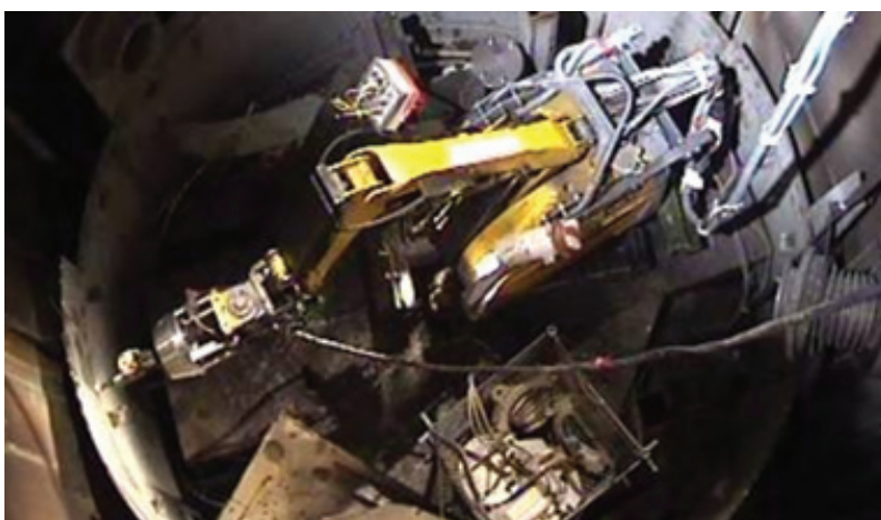
FIG. 3. Remotely operated liner removal at the SILOE research reactor in Grenoble, France.
