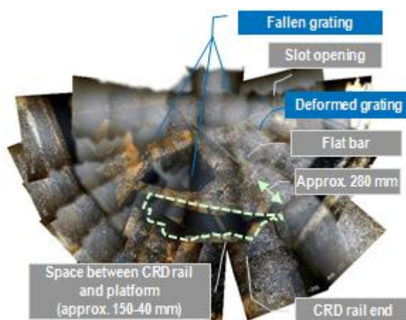
Status inside the pedestal
