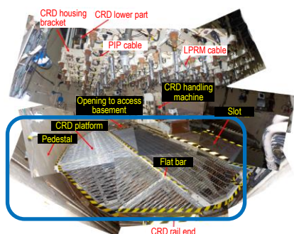
(Reference) Inside the Unit 5 pedestal
