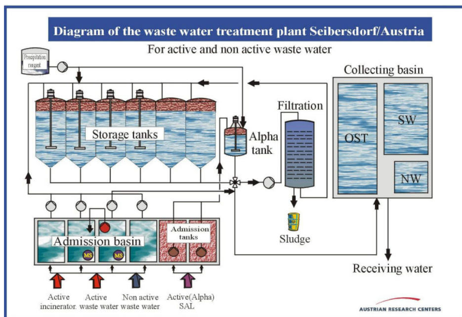
Waste water treatment plant Seibersdorf (scheme)
