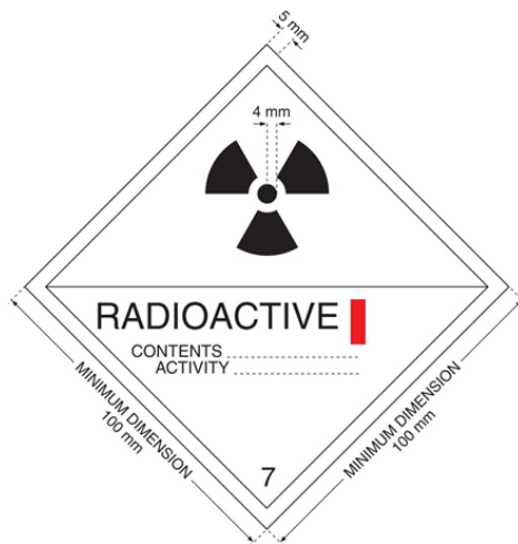
FIG. 2. Category I-WHITE label. The minimum width of the line inside the edge forming the diamond shall be 2 mm. There shall be a line inside the edge forming the diamond which shall be parallel and approximately 5 mm from the outside of the line to the edge of the label. The background colour of the label shall be white, the colour of the trefoil and the printing shall be black, and the colour of the category bar shall be red.
