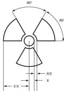
FIG. 1. Basic trefoil symbol with proportions based on a central circle of radius X . The minimum allowable size of X shall be 4 mm. For radioactive material having other dangerous properties, see para. 507.
