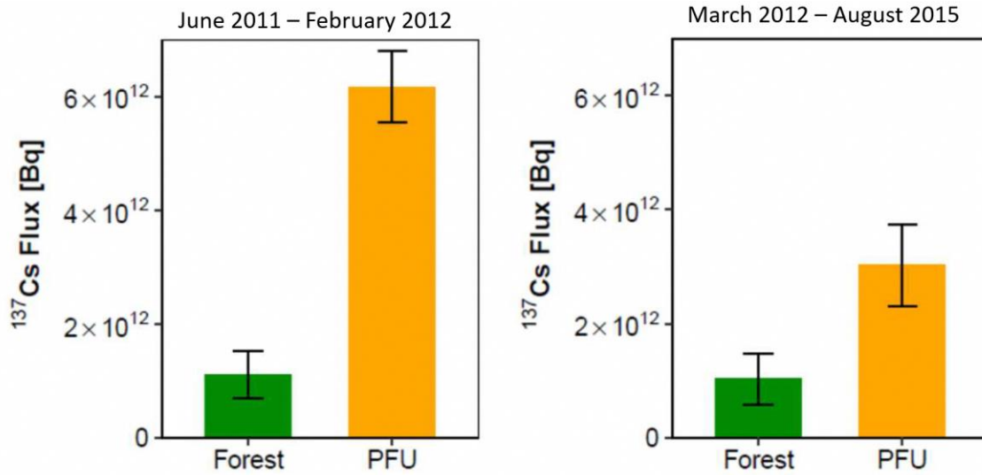
FIG. 9: Flux of particulate ^{137}\text{Cs} from forests and PFU from observed in the catchment Iwanuma (Forest: 62%, PFU 30%). Image credit: Fukushima Prefecture [15].
