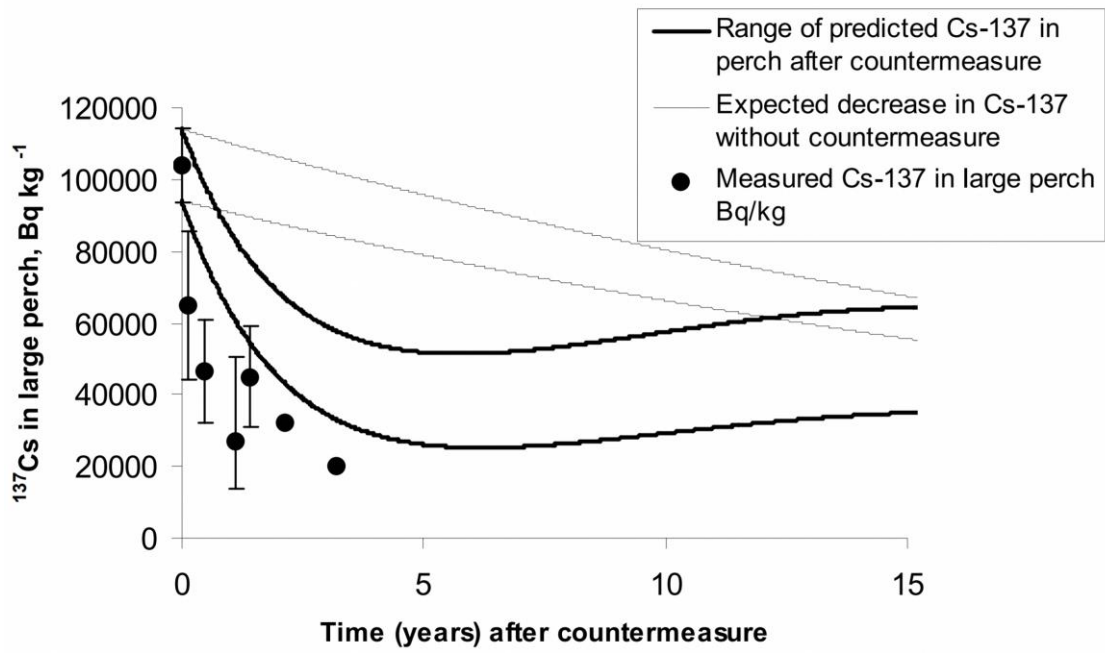
FIG. 15: Activity concentration of ^{137}\text{Cs} in perch from the potassium application in 1998 to 2013. The expected decrease in the absence of countermeasures is shown as well, an effective half-life of 20 years has been assumed [45].
