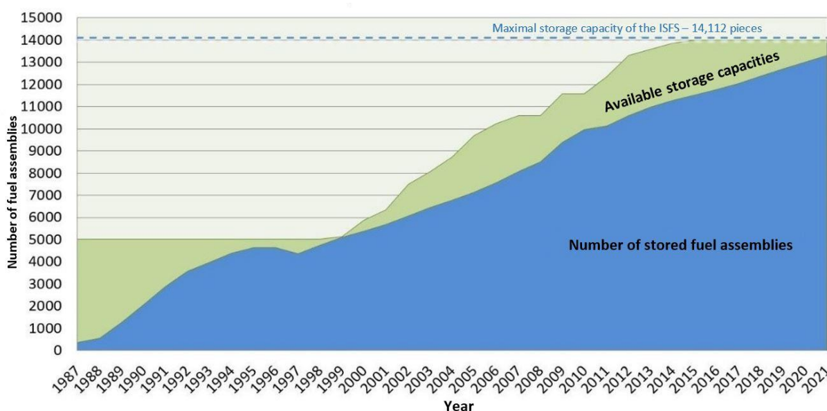
Fig. 7 Progressive filling of ISFS with spent fuel as at 31 December 2021
