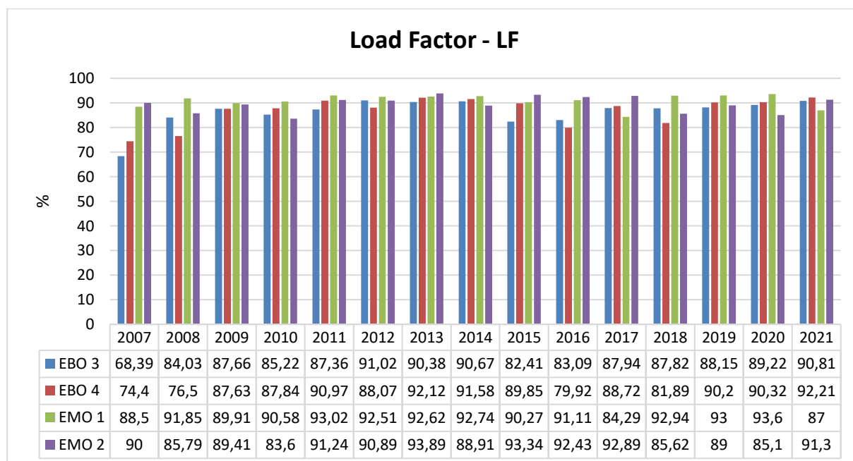
Fig. 27 Load Factor – net unit output in SE - EBO and EMO, from 2007 showing only SE, a. s. Units
