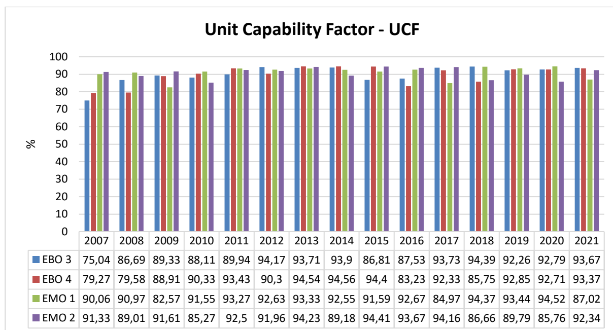
Fig. 26 Unit Capability Factor (UCF) from 2007, showing only SE, a. s. Units
