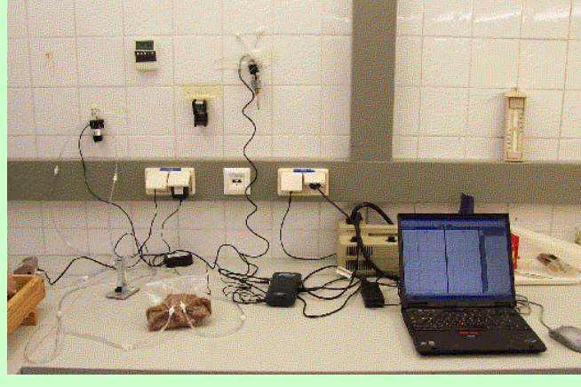
Figure 16. Equipment used for oxygen measurements
