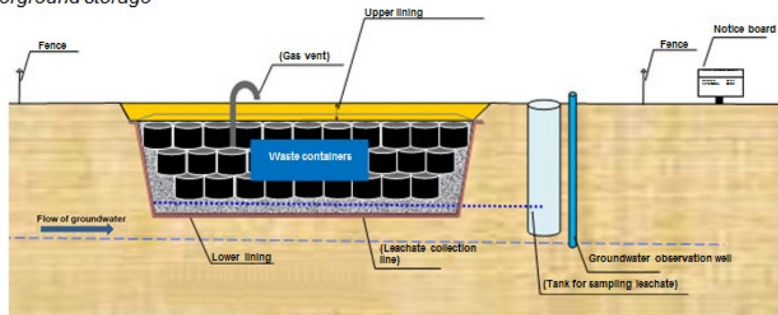
FIG. 6 Conceptual diagrams of three types of TSS (Image adapted from Technical Guidelines for temporary storage sites, Fukushima Prefecture)
