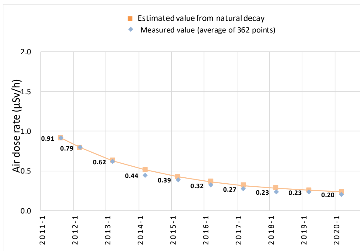
FIG 1: Measured air dose rates at 362 monitoring points in forests within the Prefecture and estimated air dose rates based on radioactive decay of radiocaesium, (Image: based on data from Fukushima Prefecture)
