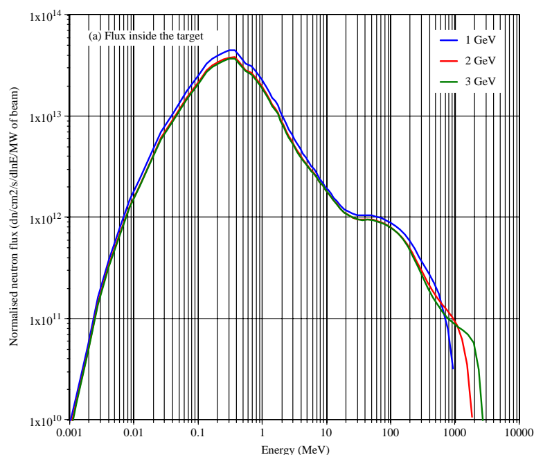
Figure 3. Neutron energy spectrum (neutrons/ \text{cm}^2/\text{s}/\text{dlnE}/\text{MW} of beam) for different proton energies, inside the Hg target.
