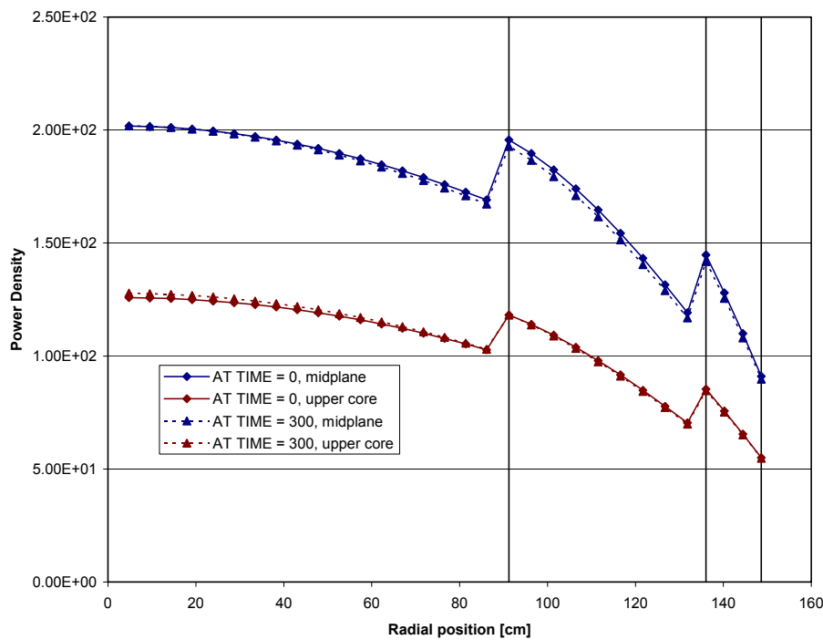
Fig.8 Radial power profiles in the core for subcycle.1
