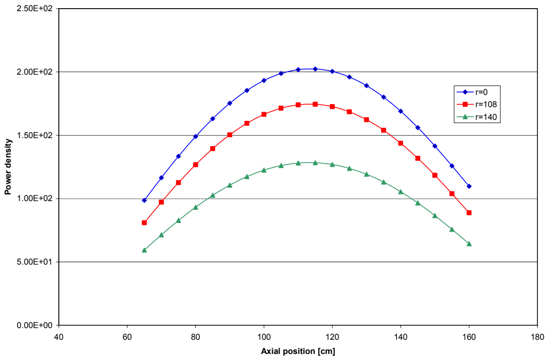
Fig.5 Axial power profiles in the core at the beginning of cycle (Tokyo Tech)
