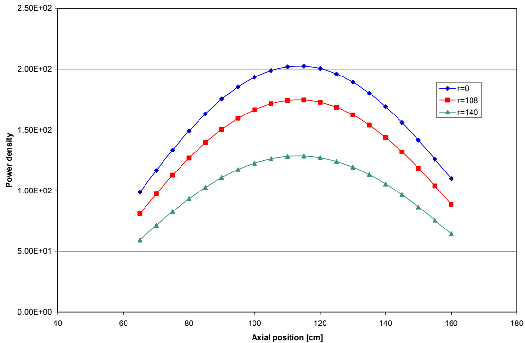
Fig.3 Axial power profiles in the core at the beginning of cycle
