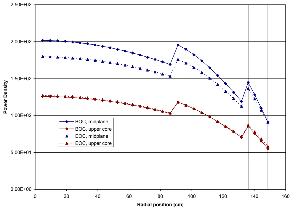
Fig.1 Radial power profiles in the core
