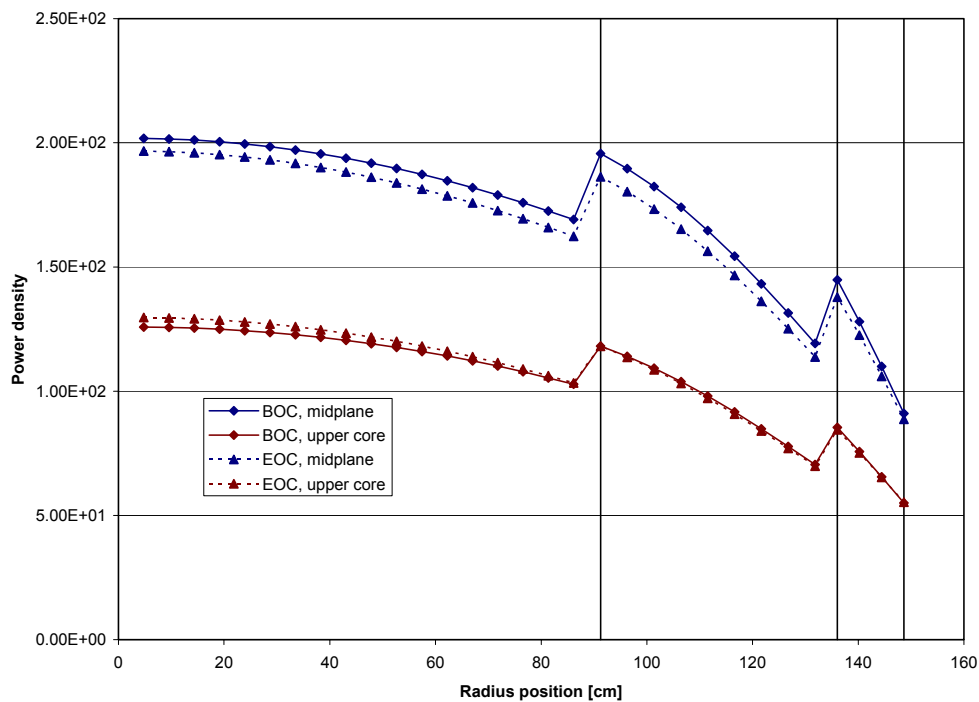
Fig.4 Radial power profiles in the core
