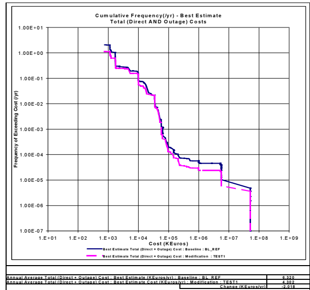
Figure 3. Risk Reduction Through Innovative NPP Safety Improvements. An example Loss curve for baseline and modification.
