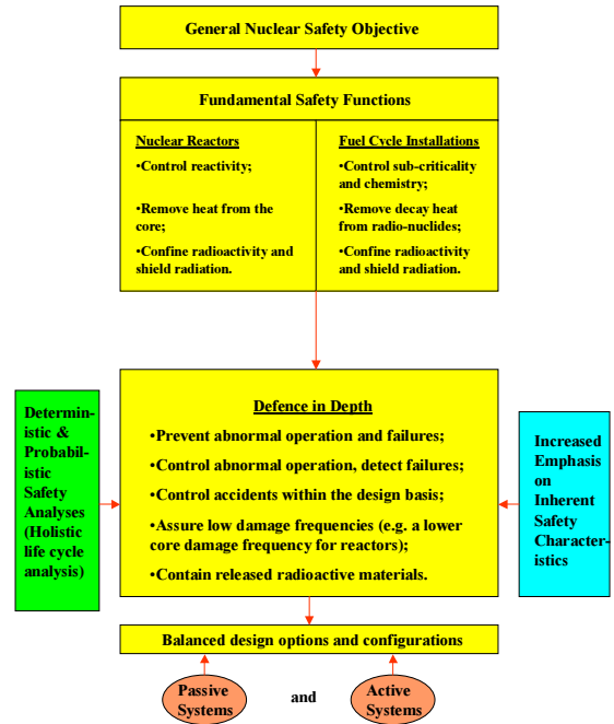
Figure 2: Framework for development of requirements for safety of INS
