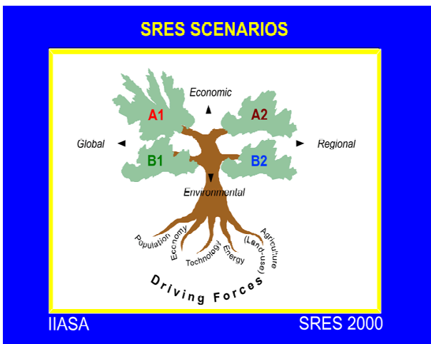
Figure 2: SRES scenarios used in INPRO
