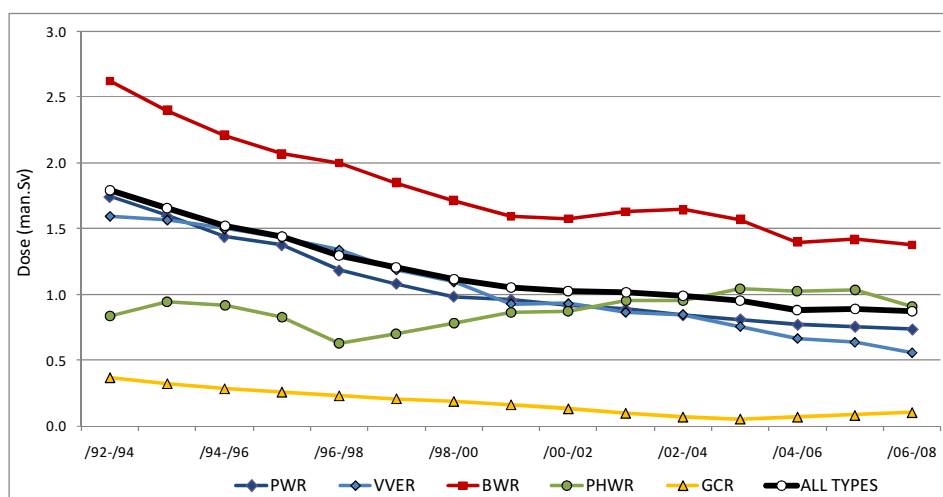
Figure 4: Three-year rolling average collective dose by reactor type for all operating reactors in the Information System on Occupational Exposure (ISOE), 1992–2008 (man·Sv) [pressurized water reactor (PWR); boiling water reactor (BWR); water cooled water moderated power reactor (VVER); pressurized heavy water reactor (PHWR); gas cooled reactor (GCR); light water cooled graphite moderated reactor (LWGR)] Reference: ISOE Occupational Exposure Database 2009, (co-sponsored by the OECD/NEA and IAEA)
