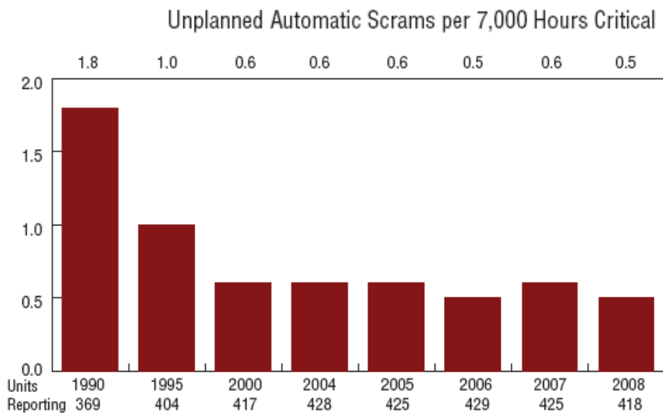
Figure 3: Unplanned automatic scrams per 7000 hours critical (source: 2008 Performance Indicators World Association of Nuclear Operators)
