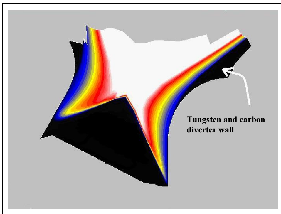
FIG. C-1. Computer simulation of the temperature profile of the diverter region of a fusion device. Temperatures range from ~ 200 000 (blue) to 1 000 000 (red) Kelvin, close to the temperature at the centre of the sun. Calculated with the B2-IRENE computer model (Research Centre Jülich), this study required voluminous reliable atomic and molecular data, many of which have been derived and assembled from a series of recent Agency coordinated research projects.
