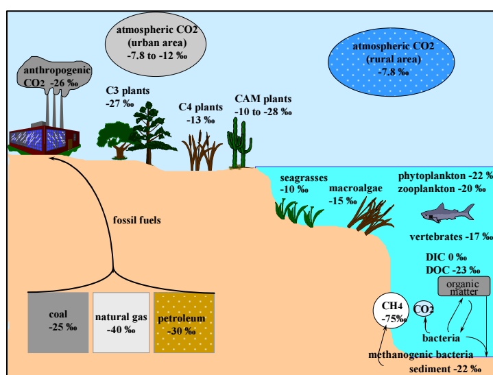
FIG. G-3. Schema of \delta^{13}\text{C} distribution in the environment (modified figure after Tolosa, Oceanis , vol. 30 n.2, 2004, pp. 239–259) (CAM = crassulacean acid metabolism; DIC = dissolved inorganic carbon; DOC = dissolved organic carbon).
