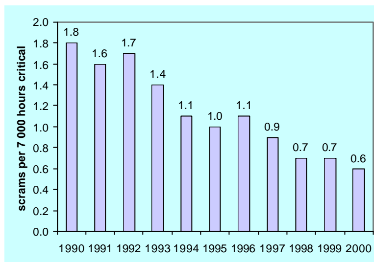
Figure II-1. Unplanned automatic scrams per 7 000 hours critical
