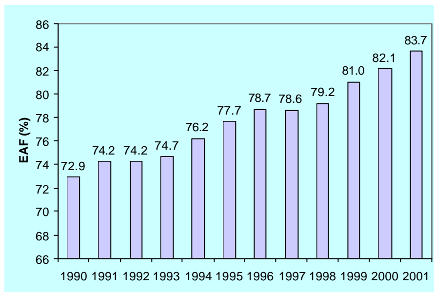
Figure II-4. Global average energy availability factor (EAF)
