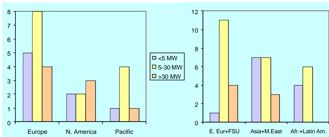
Figure I-4. Number and power distribution of isotope-producing reactors in OECD and non-OECD Countries
